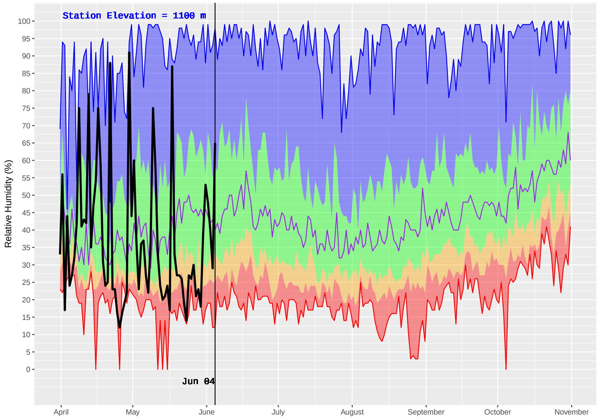
PALLISER (411) : Historical (1973–2016) and Current (2018) Noon Relative Humidity
