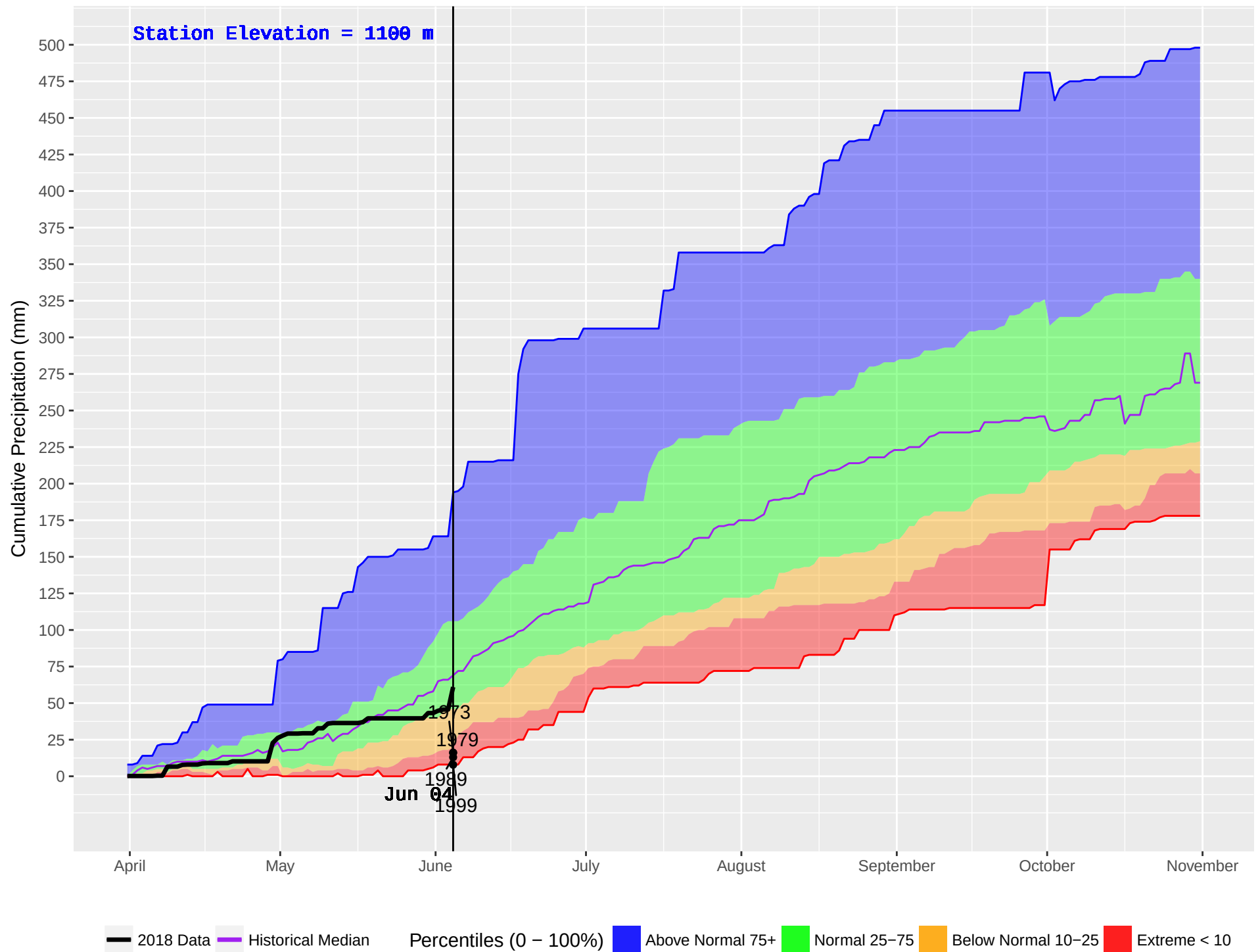
PALLISER (411) : Historical (1973–2016) and Current (2018) Noon Cumulative Precipitation
