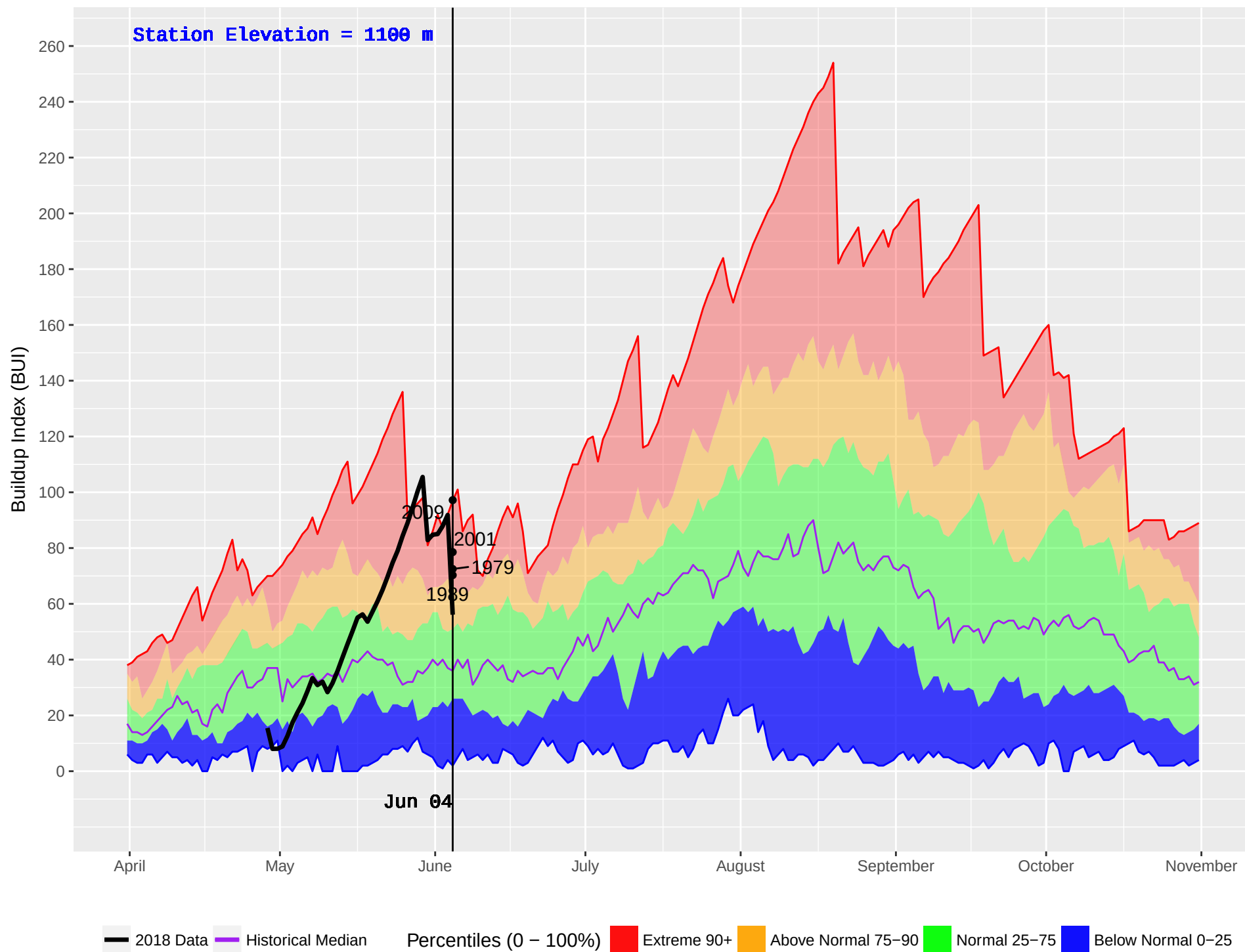
PALLISER (411) : Historical (1973–2016) and Current (2018) Noon Buildup Index (BUI)
