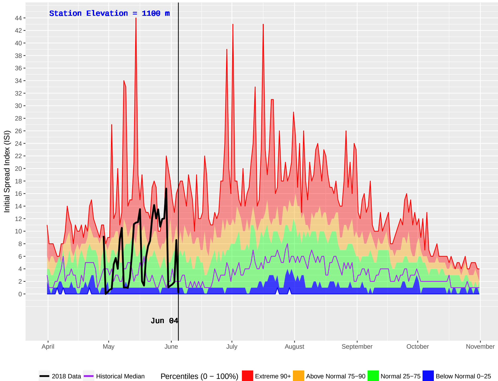
PALLISER (411) : Historical (1973–2016) and Current (2018) Noon Initial Spread Index (ISI)
