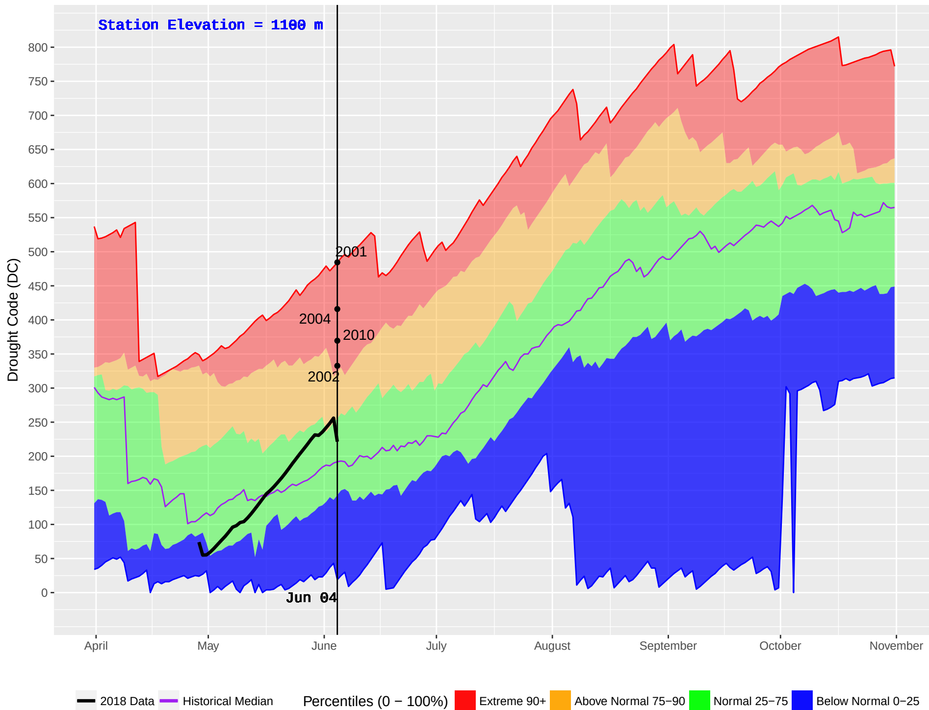
PALLISER (411) : Historical (1973–2016) and Current (2018) Noon Drought Code (DC)
