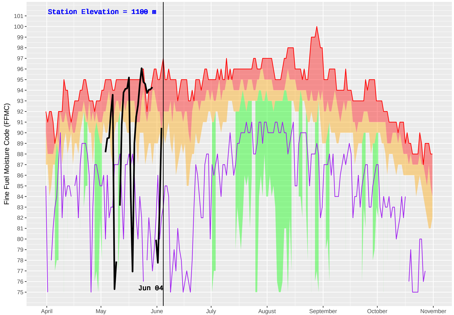
PALLISER (411) : Historical (1973–2016) and Current (2018) Noon Fine Fuel Moisture Code (FFMC)
