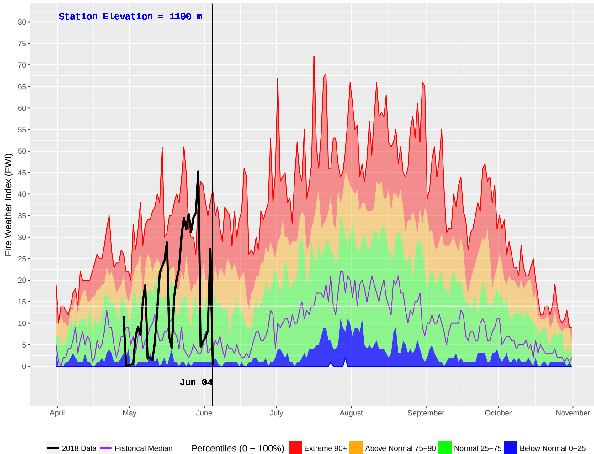
PALLISER (411) : Historical (1973–2016) and Current (2018) Noon Fire Weather Index (FWI)
