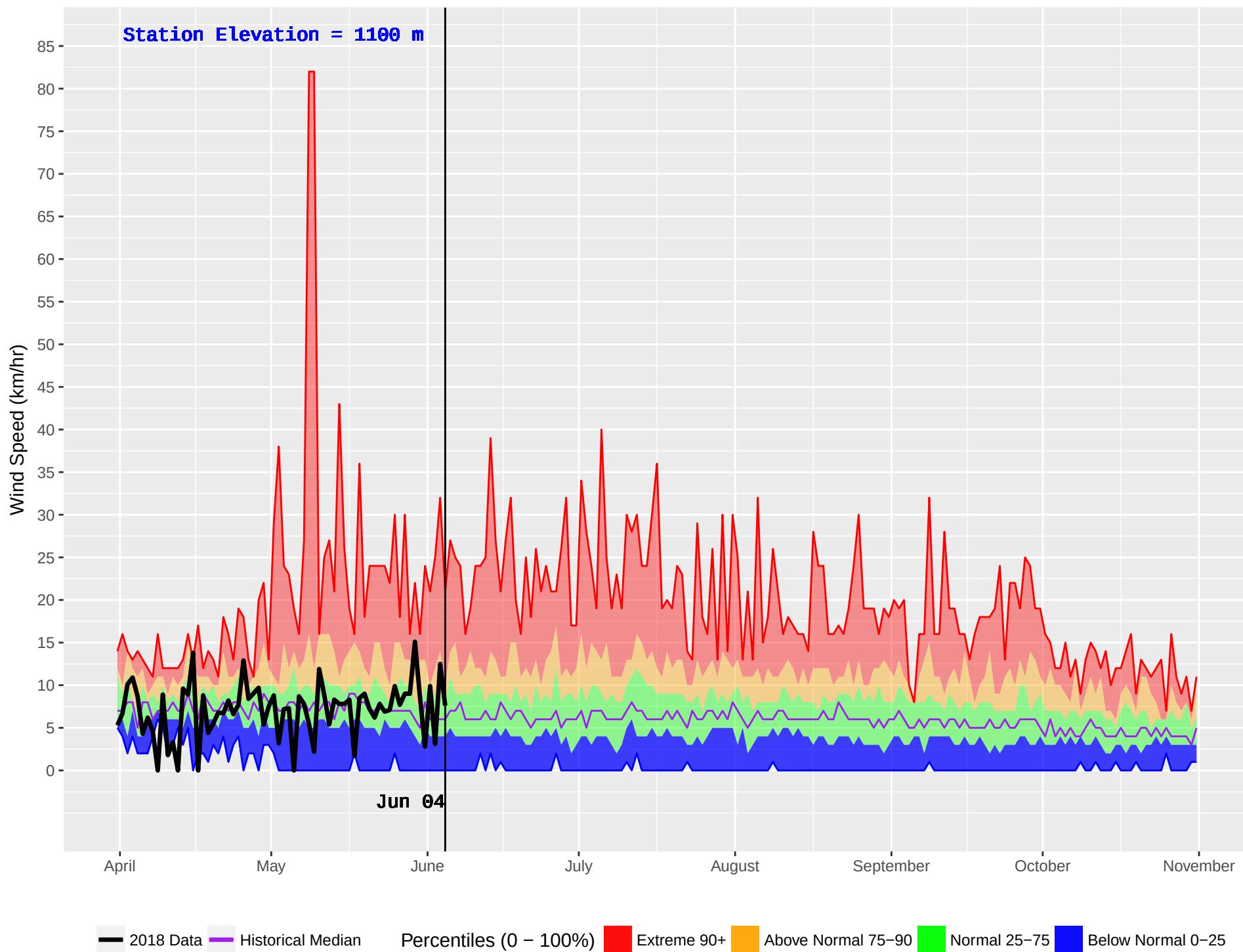
PALLISER (411) : Historical (1973–2016) and Current (2018) Noon Wind Speed
