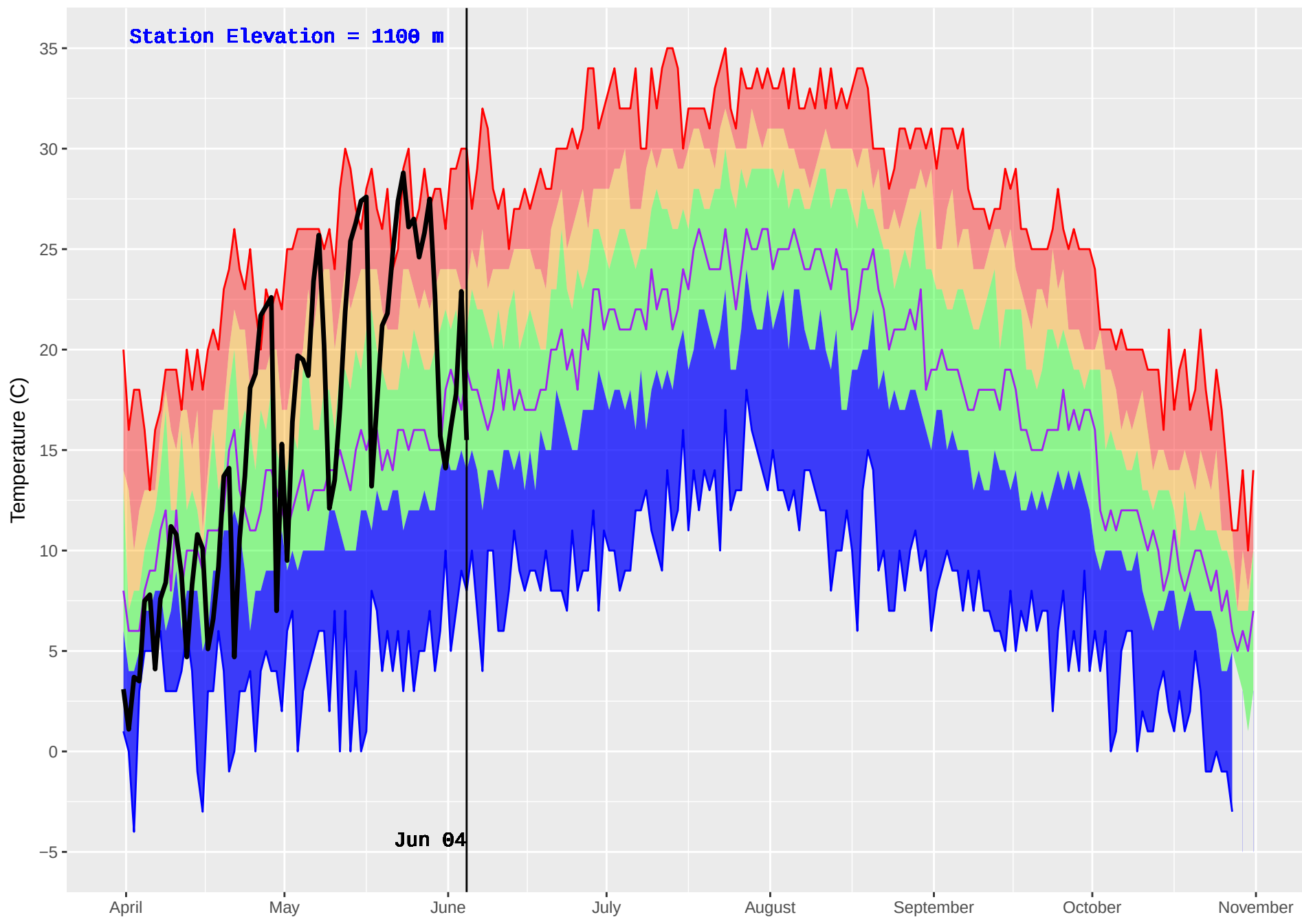
PALLISER (411) : Historical (1973–2016) and Current (2018) Noon Temperature
